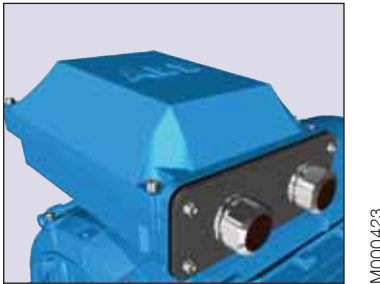
Fig 2. Terminal box for motor sizes 280-315 with connection flange and cable glands.
