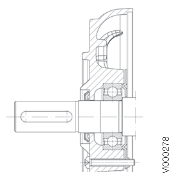
Motor sizes 71-132
