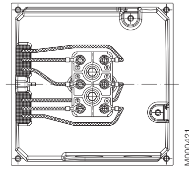
Terminal board for motor sizes 132
