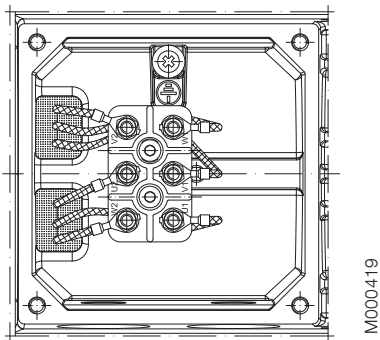
Terminal board for motor sizes 071-080
