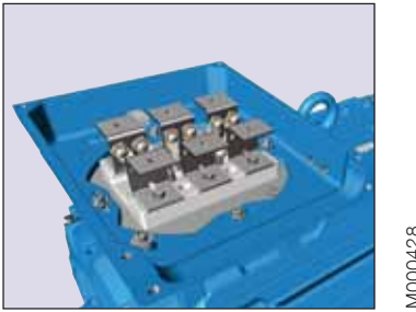
Fig 7. Terminal board for motor sizes 355-400.
