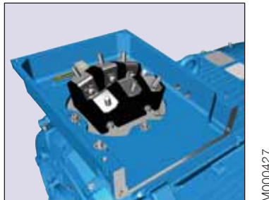
Fig 6. Terminal board for motor sizes 280-315.
