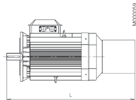
Separate cooling with or without tacho Variant codes; 183, 474, 476, 477, 189, 574, 576 and 577
