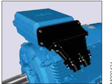
Fig 3. Terminal box for motor sizes 355-400, with adapter and cable sealing end unit.
