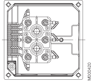
Terminal board for motor sizes 090-112
