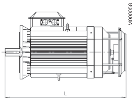
Tacho Variant codes; 472, 473, 572 and 573
