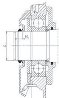
V-ring
