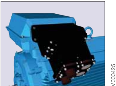
Fig 4. Terminal box for motor sizes 450, with adapter and cable sealing end unit.
