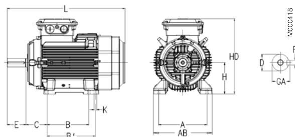
Foot-mounted motor IM1001, B3
